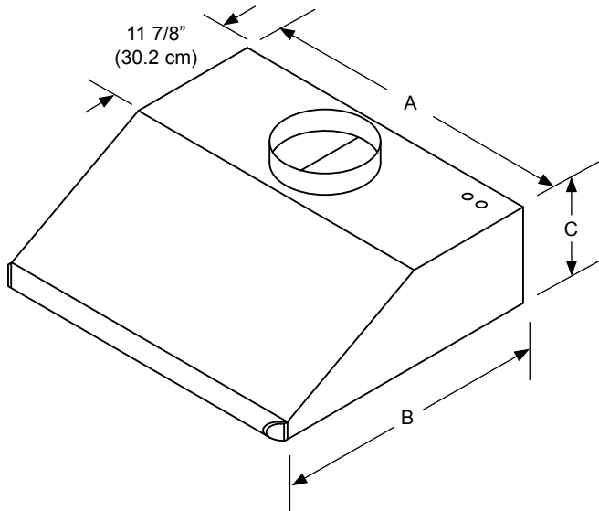
OVERALL DIMENSIONS
