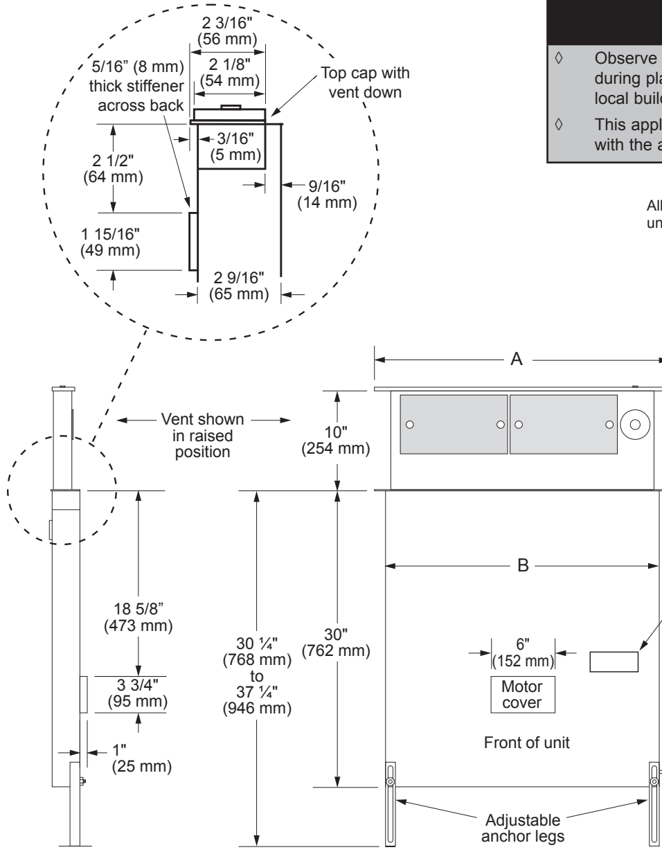
DIMENSIONS SIDE VIEW
