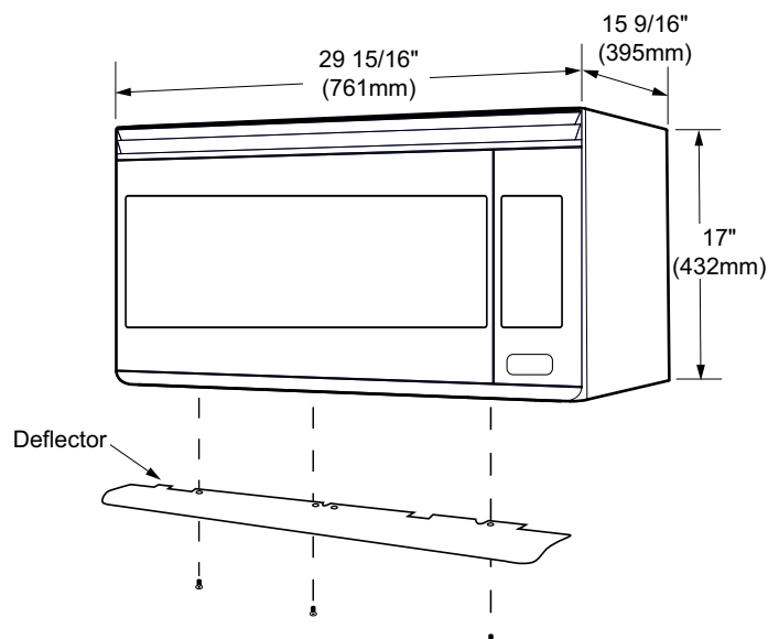
OVERALL DIMENSIONS
