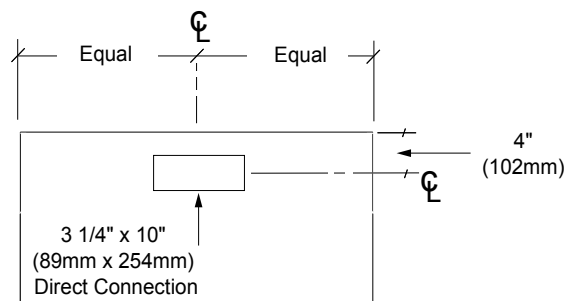
MICROWAVE TOP VIEW EXHAUST LOCATION
