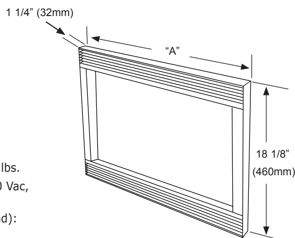
AOMTK OVERALL DIMENSIONS (Preference® Trim Kit)
