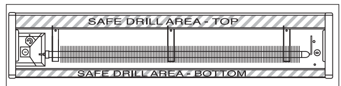
Drill areas; left end wiring shown
