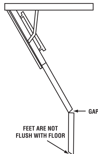
FIGURE 8C - INCORRECT SETUP
