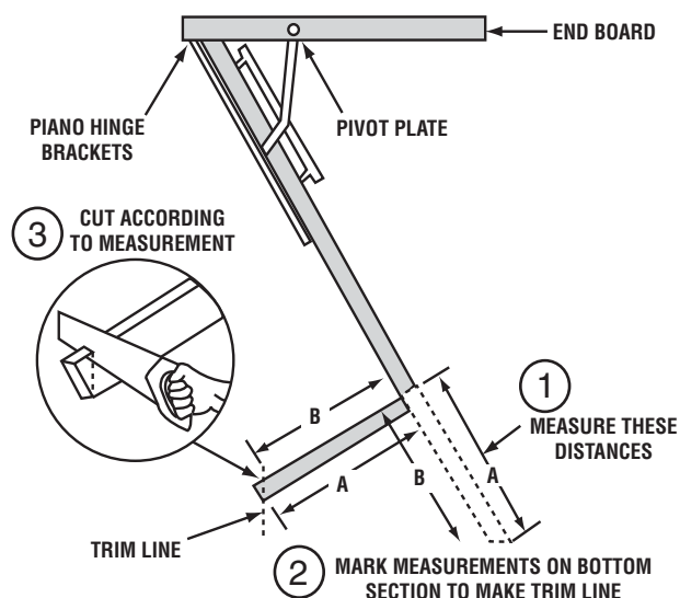
FIGURE 7A - ADJUSTMENT TO CEILING HEIGHTS
