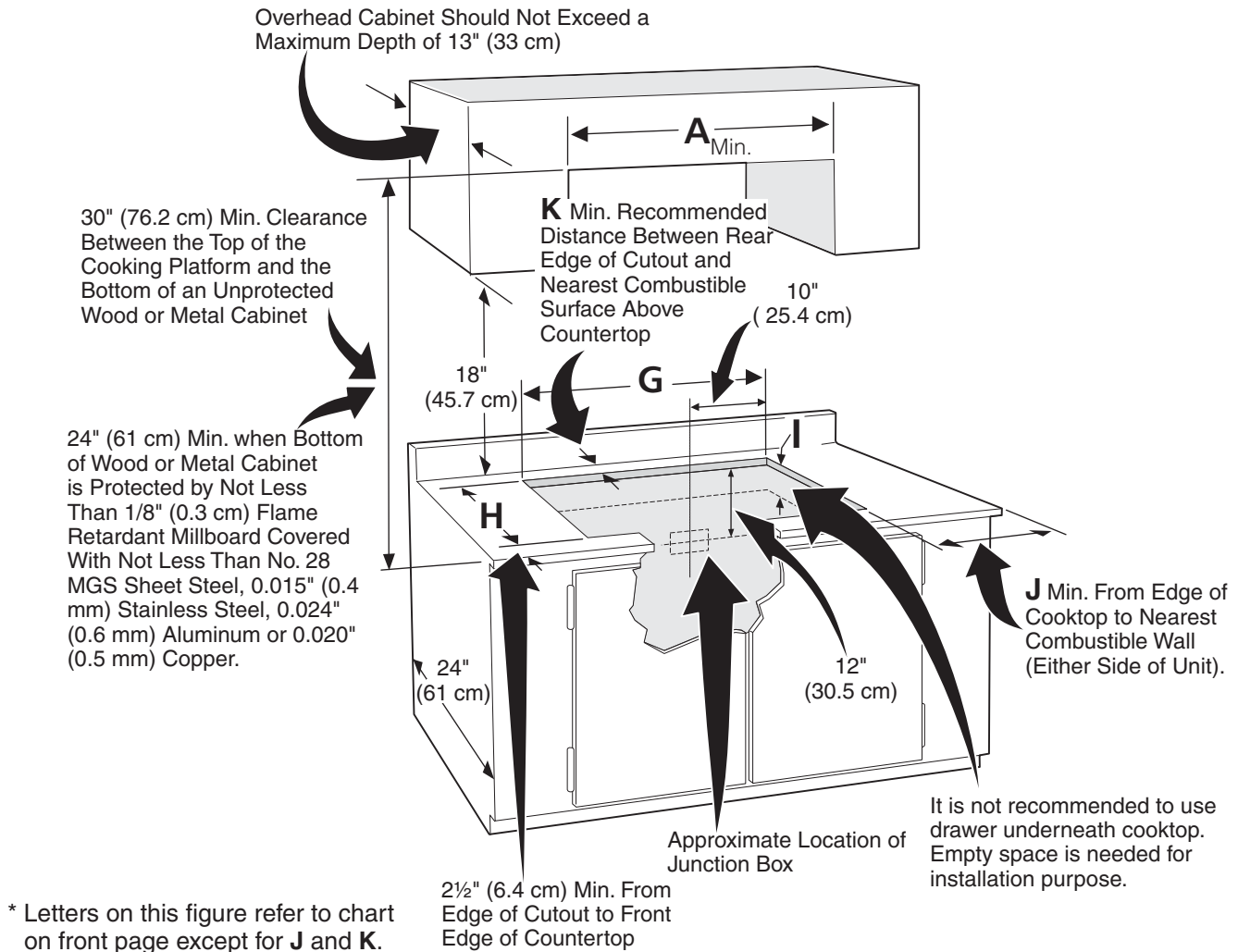
Figure 2 – COUNTERTOP CUTOUT OPENING
