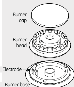
Front right burner (on some models)
