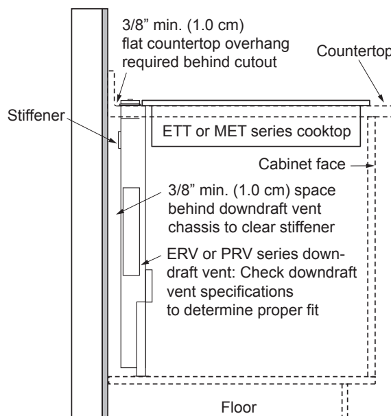
Side View: Cooktop and ERV/PRV Series Downdraft
