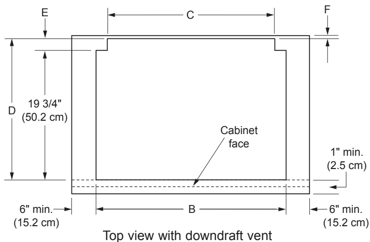
Dimension Table - Installations with Downdraft Vent
