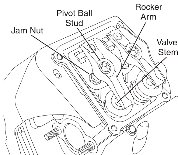
Figure 23 - Valve Clearance Adjustment
