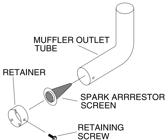
Figure 22 - Spark Arrestor
