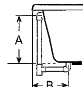
DRAIN/OVERFLOW
