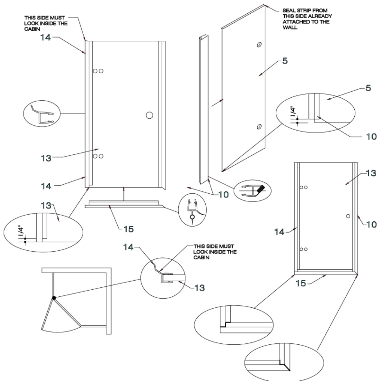
FIG.7 SEAL STRIP INSTALLATION
