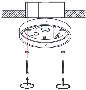
Wooden Ceiling
