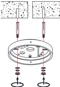
Concrete ceiling
