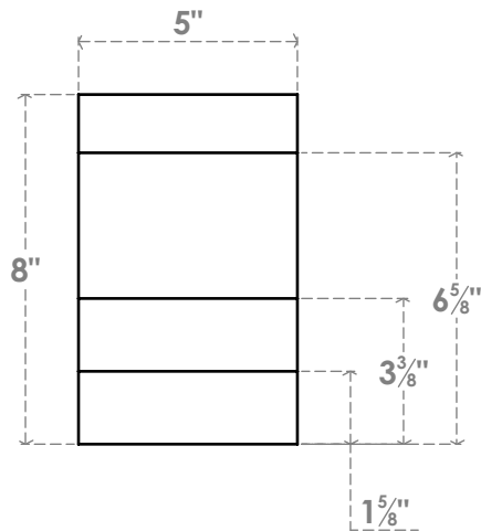
FRONT PROFILE
