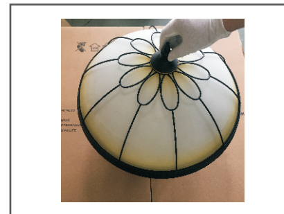
Step 8. Fasten the decorative accessories to the screw. As is shown in the figure.
