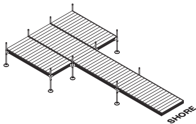
24' PLATFORM DOCK (5 Sections)
