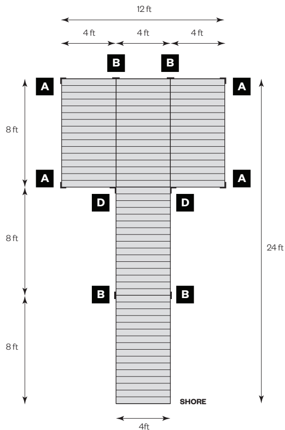
24' PLATFORM DOCK
