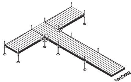
24' PLATFORM DOCK (6 Sections)
