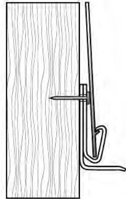
Fig. 2 Undersill with Snaplock and Flashing
