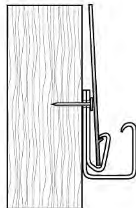
Fig. 3 J-Channel and Undersill Trim
