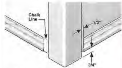
Fig.1 Standard Corner Post
