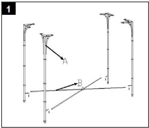
Step 1 Assemble the Legs(A) Stretcher(B) together using 4 Screws.
