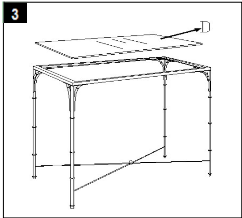
Step 3 Carefully place the Glass Top(D)
