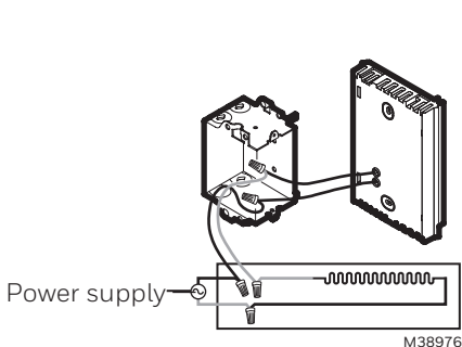
2-wire Installation
