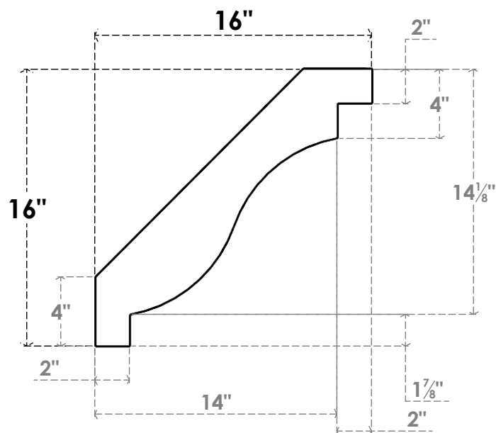
SIDE PROFILE
