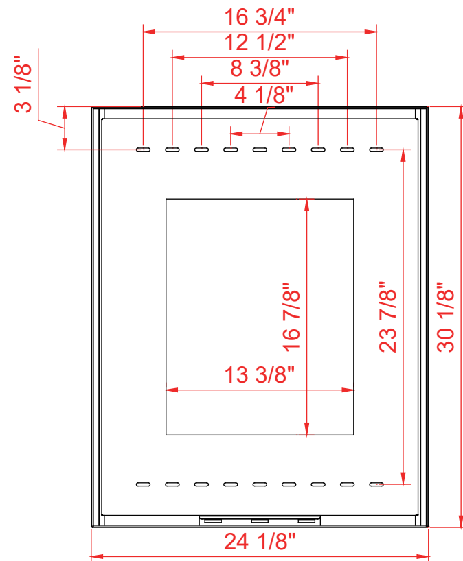
BACK VIEW
