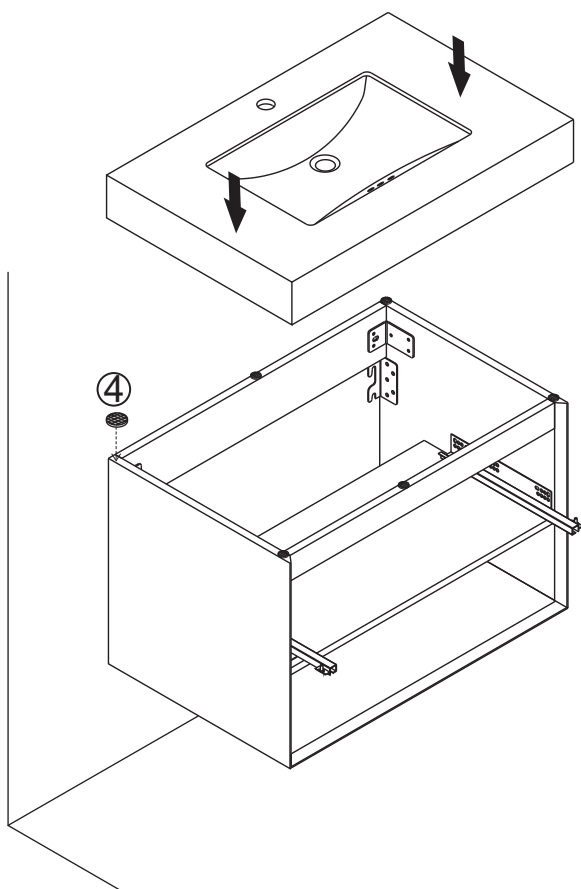
Installation of drain assembly
