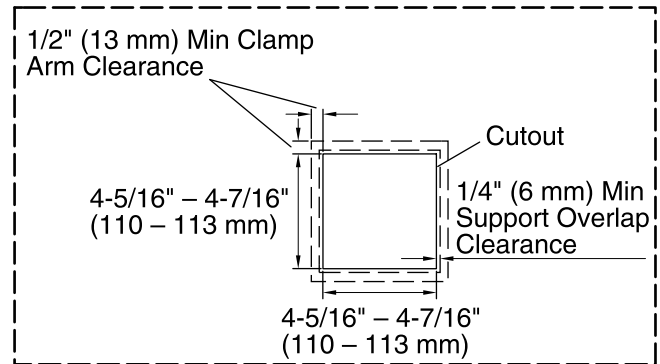
Cutout Detail
