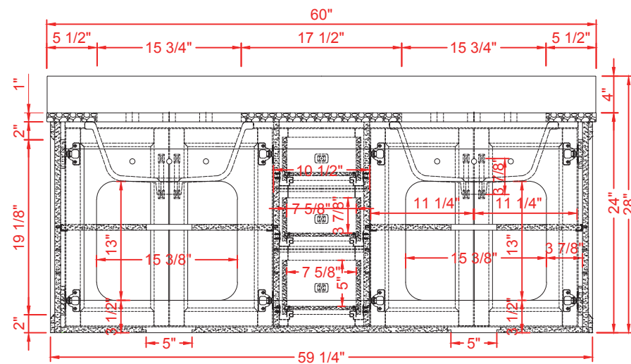
BACK VIEW
