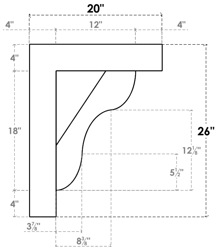
SIDE PROFILE
