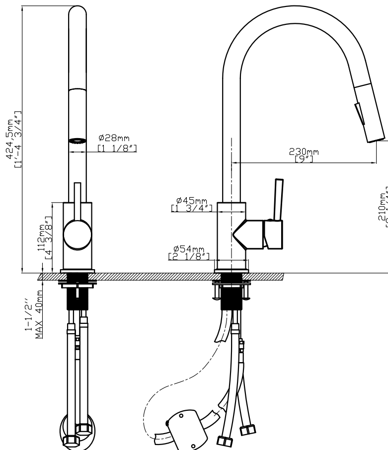
CRITICAL DIMENSIONS
