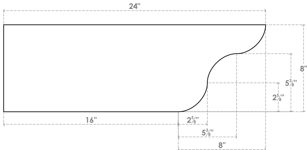
SIDE PROFILE
