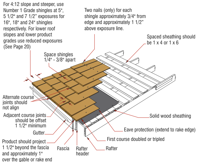
Figure 5: Certi-label Shingle Application
