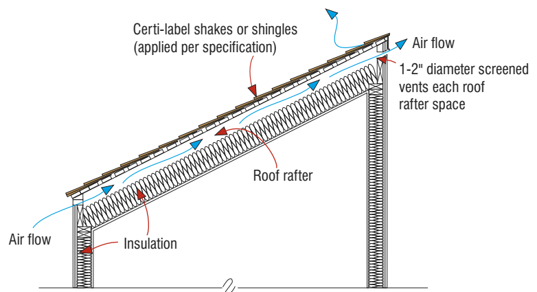
Figure 15c: Shed Roof
