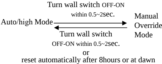
FIG.1 Manual Override Operating Diagram
