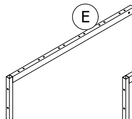
Side Rail T953320 X 2
