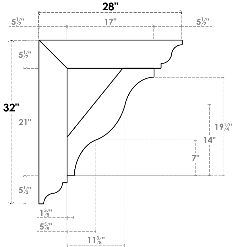
SIDE PROFILE
