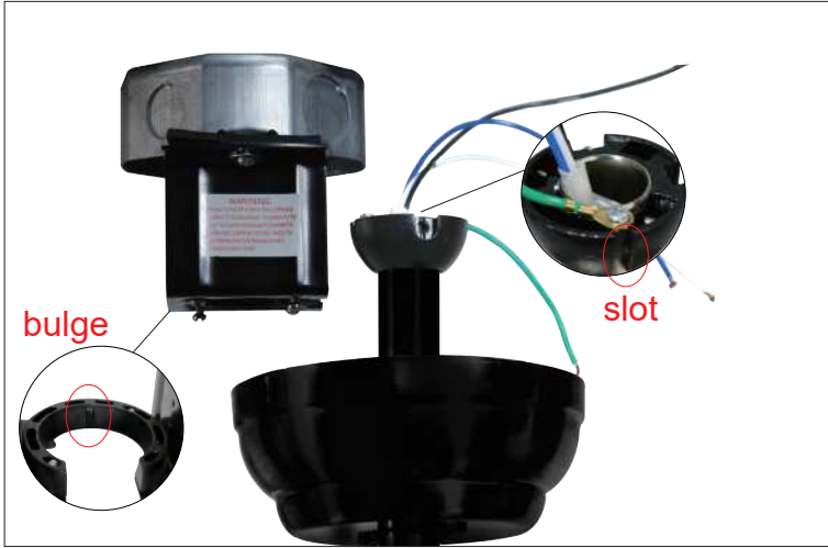
Step 11 Hang the fan on the hanging bracket and align the slot on the downrod with the bulge on the hanging bracket.
