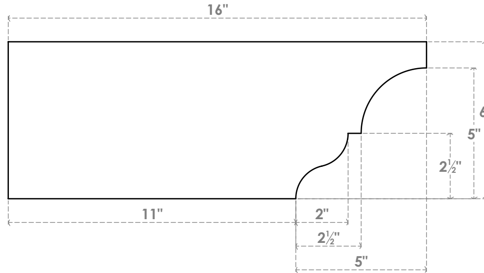
SIDE PROFILE
