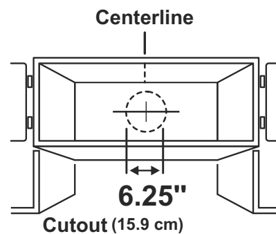
Wall/side cutout (B)
