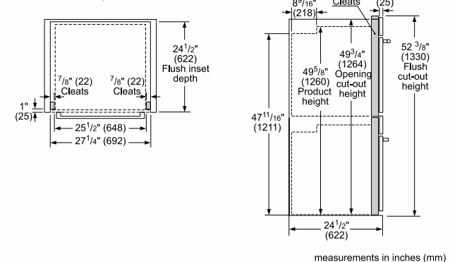
Flush installation Top view
