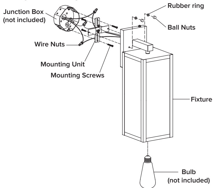
Mounting Unit
