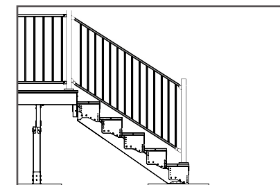
6. Mount Stair Posts & Panels (Optional)
