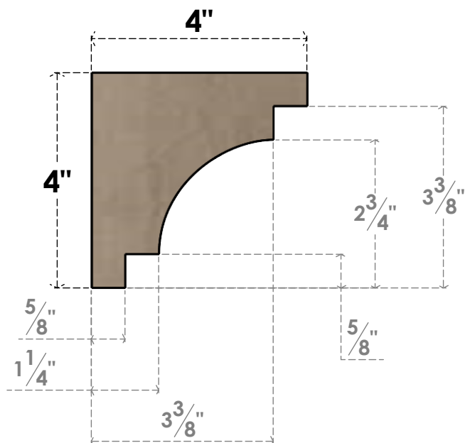
SIDE PROFILE
