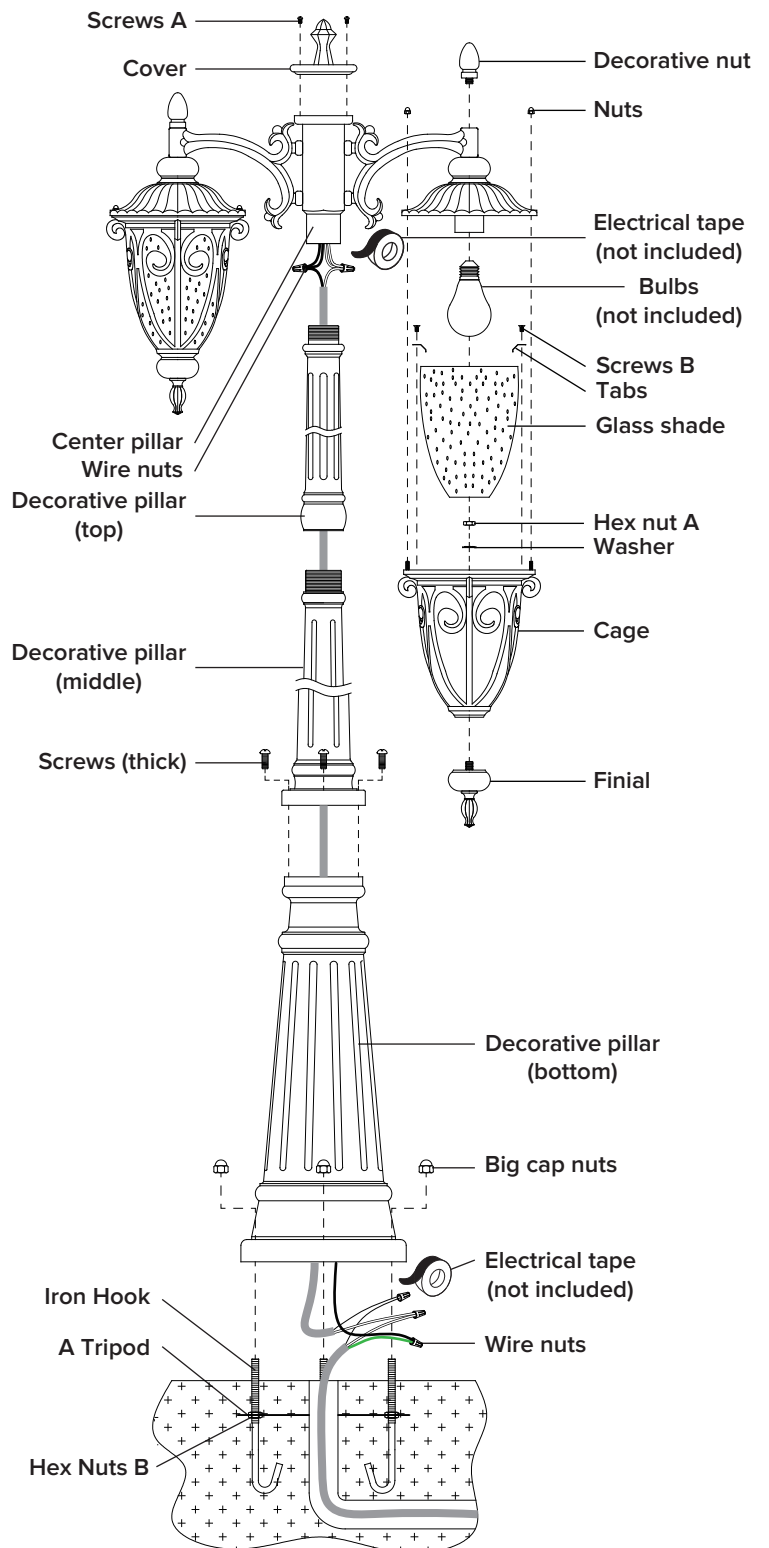
Finial (Hex nuts A, Washer)
