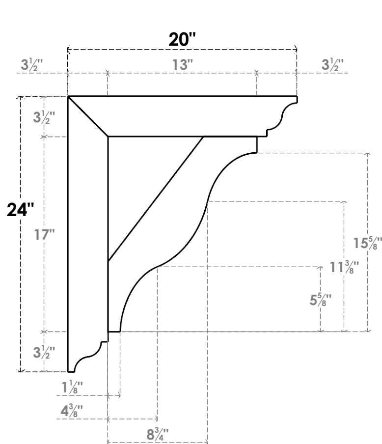
SIDE PROFILE
