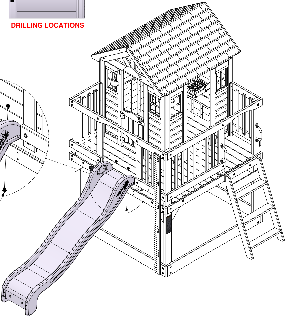
379 (x2) T-NUT - 5/16"
