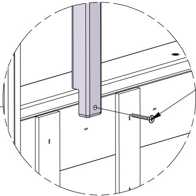
387 (x8) SCREW - 1 1/4"
