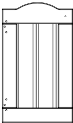
DP1 RIGHT DOOR PANEL - W2A03865 (x1) 1 1/8"x19 1/8"x11 3/8" (27x486x288)
