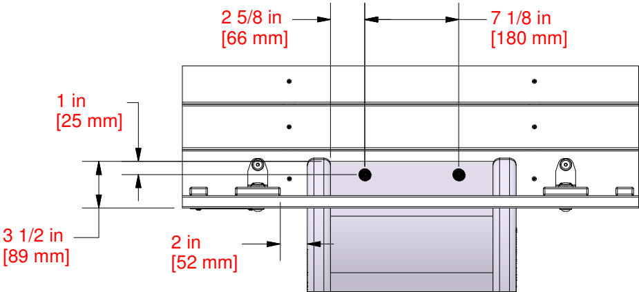
DRILLING LOCATIONS
