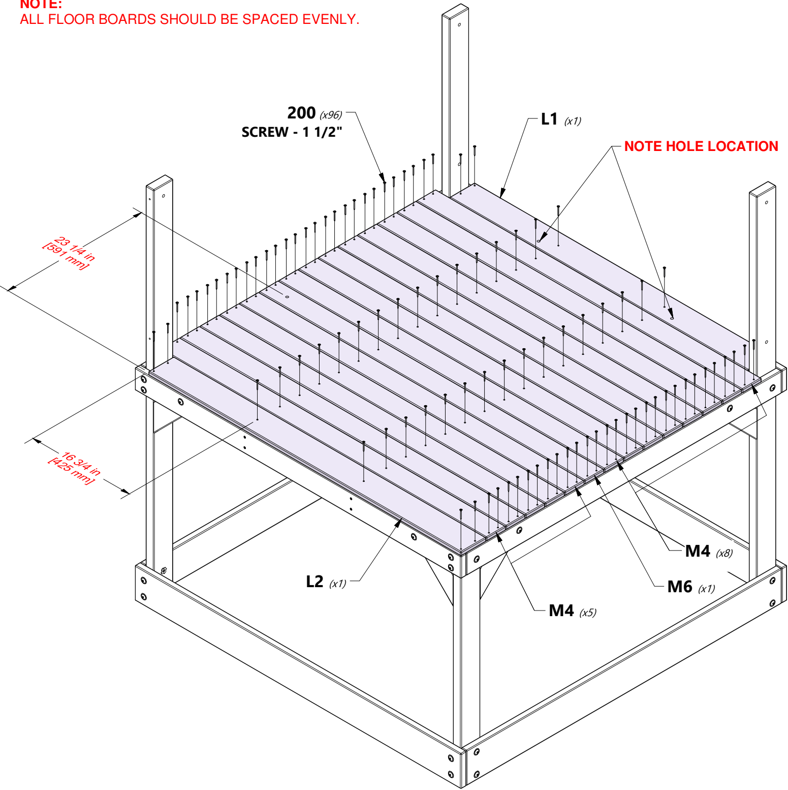
L2 FLOOR BOARD - W4L17861 (x1) 5/8"x4 3/8"x54 3/8" (16x112x1382)
