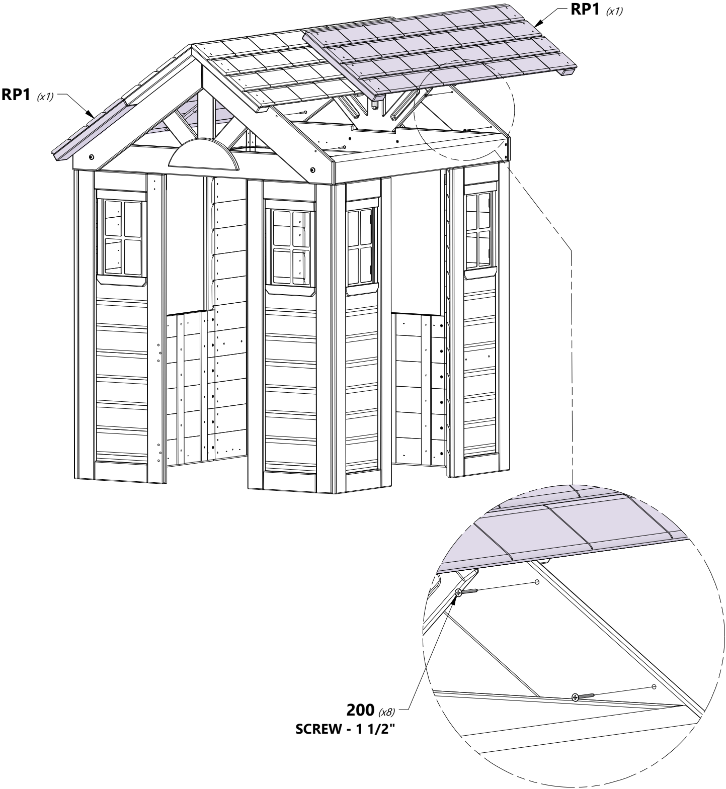
RP1 LOWER ROOF PANEL - W2A03863 (x2) 1 3/8"x13"x44 7/8" (35x329x1140)
