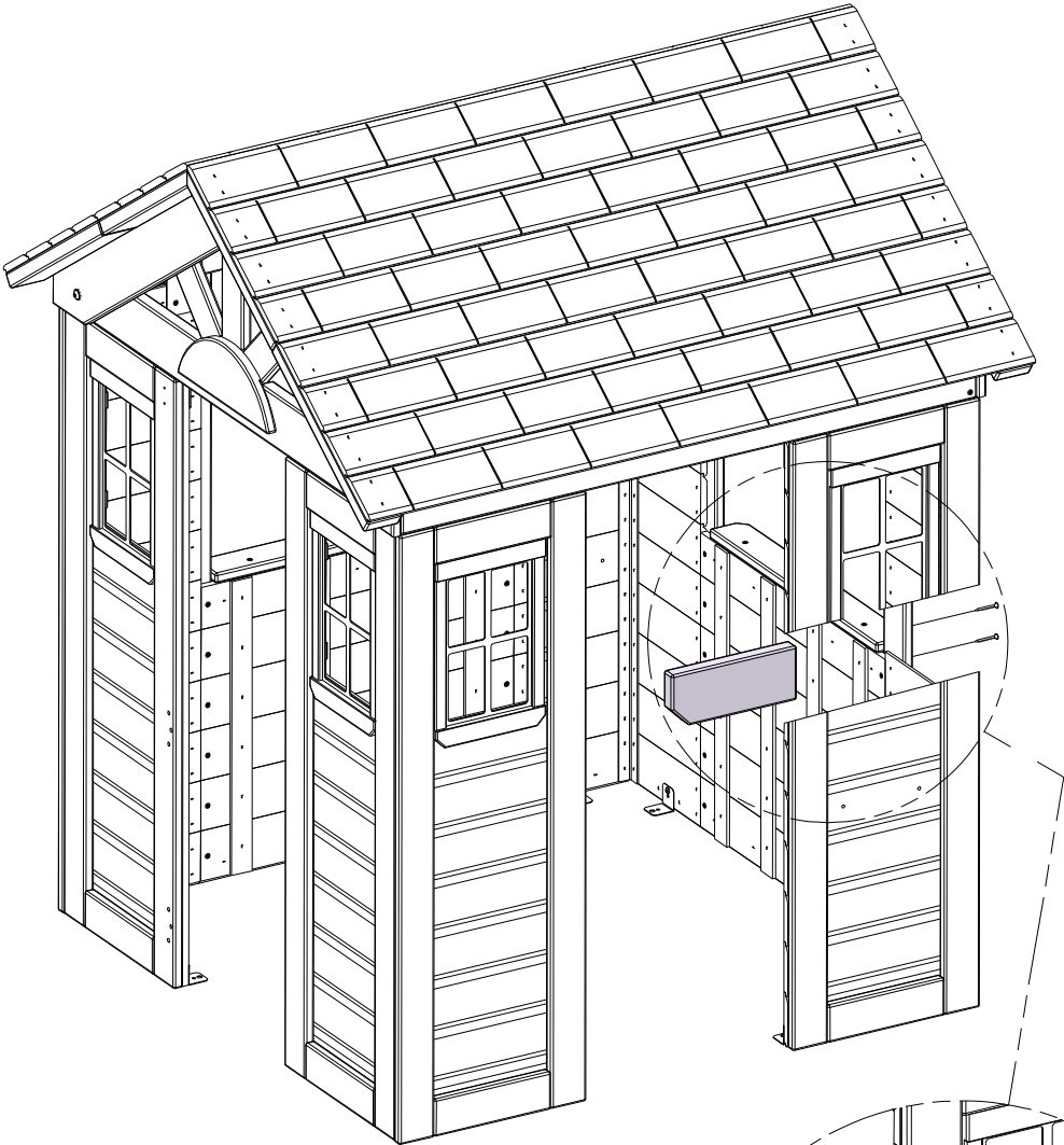
H3 COUNTER TOP SUPPORT - W4L17873 (x1) 1"x3 3/8"x8 3/8" (24x86x214)
