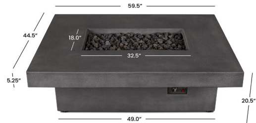
Smoke (1586LP-SMK)
