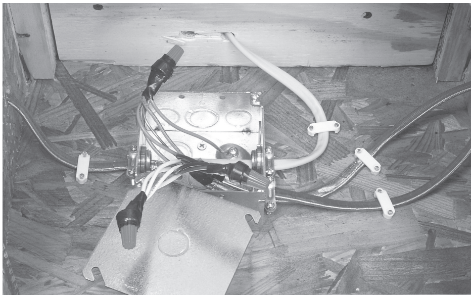
Junction box with multiple sets of mat lead wires, connected in parallel, and connected to the power supply.
