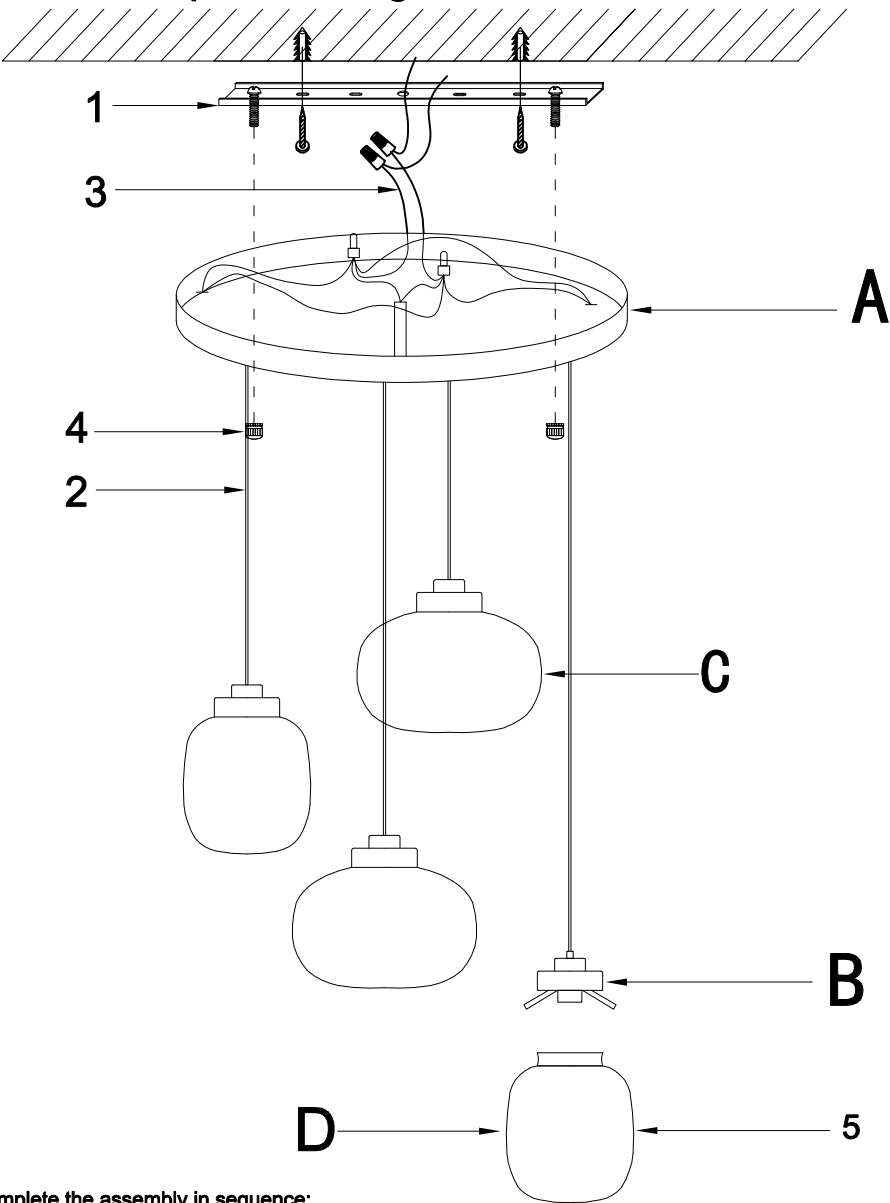
Installation sequence diagram
