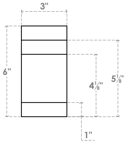
FRONT PROFILE
