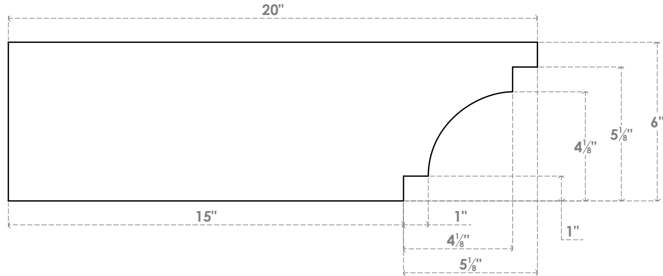
SIDE PROFILE
