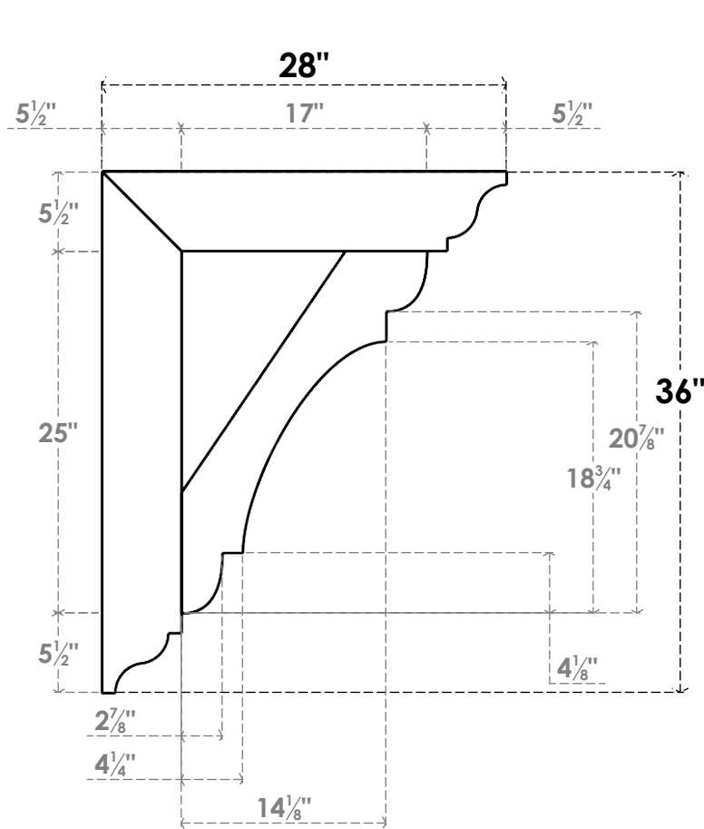
SIDE PROFILE
