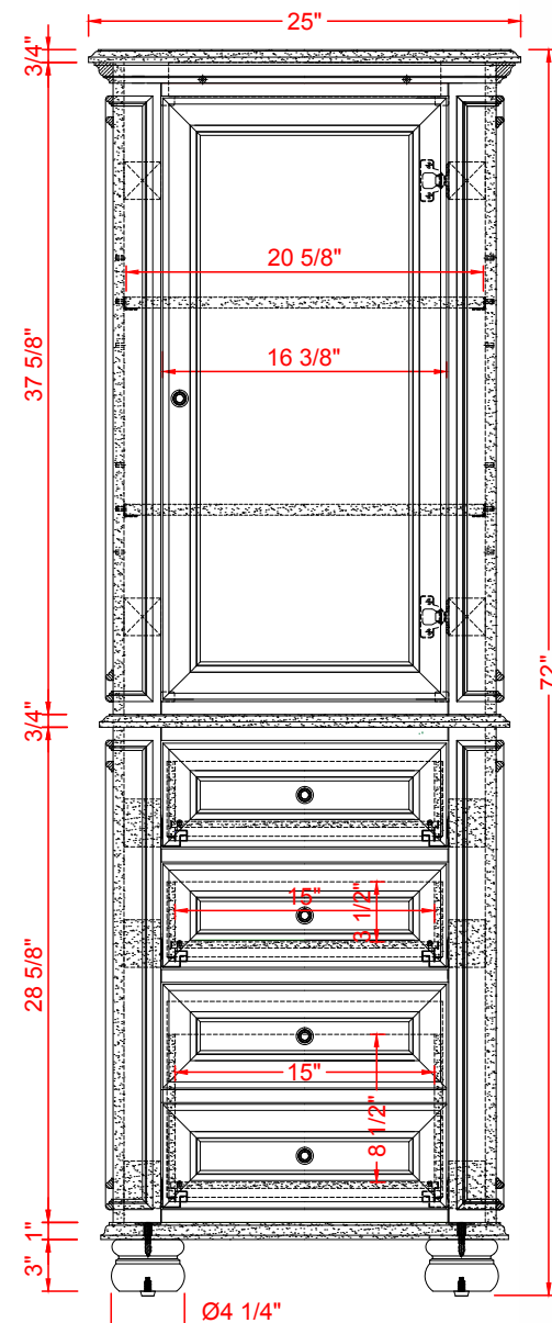
FRONT VIEW
