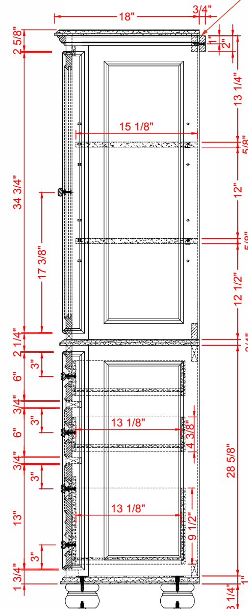
SIDE VIEW
