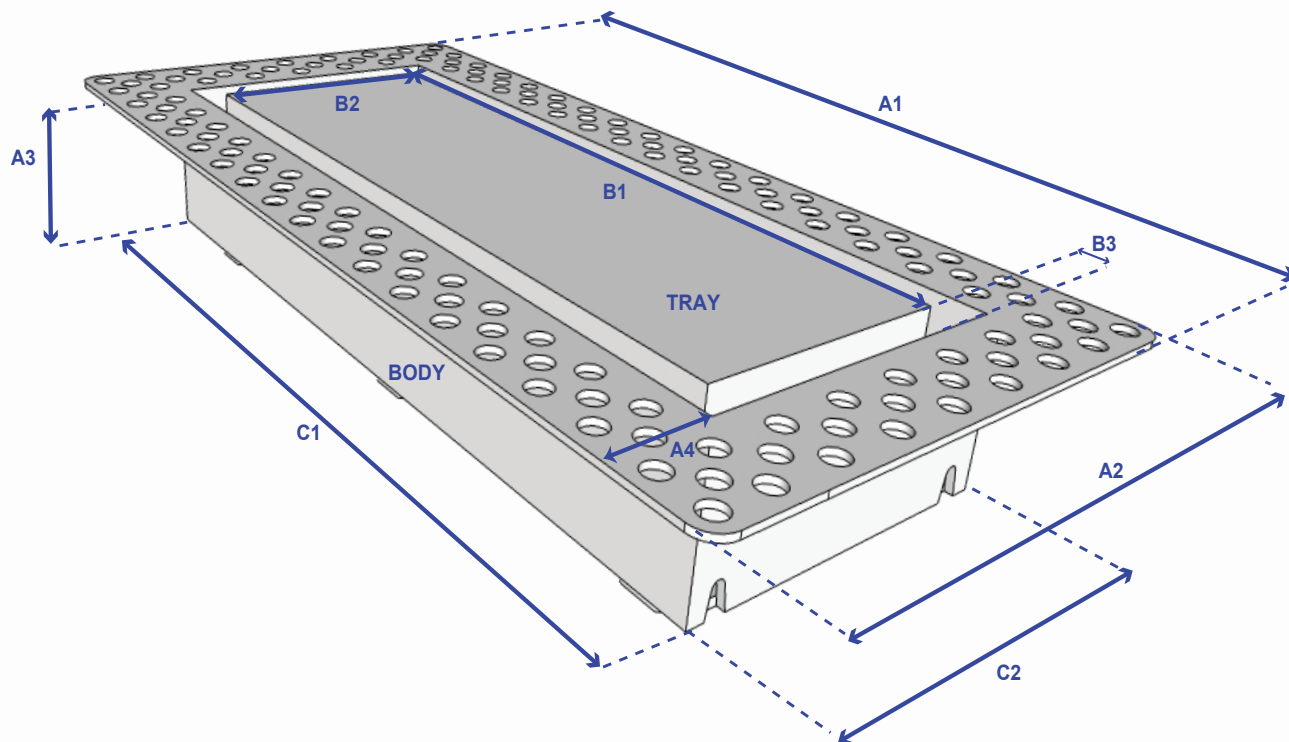
Perspective View
