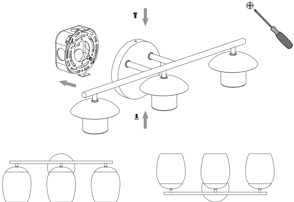
Installation Option 1: Down light
