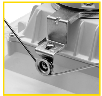
Butterfly Spring
