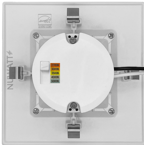
5 Kelvin Selectable
